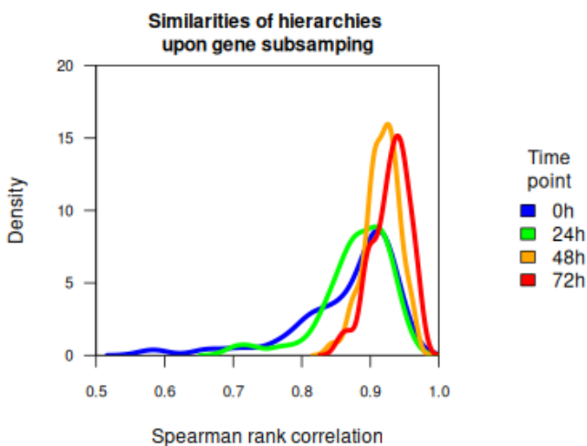
Figure 7: Similarities of hierarchies upon random gene subsampling. The figure represents the similarities between a given cell-state hierarchy and the hierarchies obtained when random sets of genes are subsampled. Four distributions are plotted corresponding to the hierarchies obtained from the libraries at different time points: 0,24,48 and 72 hours, as indicated in the legend. A high median and a low variance are indicative of a cell-state hierarchy robust to variations in the data. See text for details.
