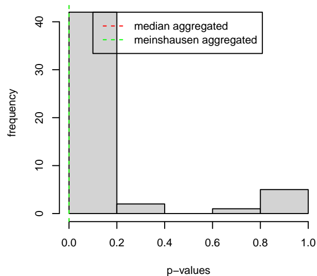
histogram single-split p-values
