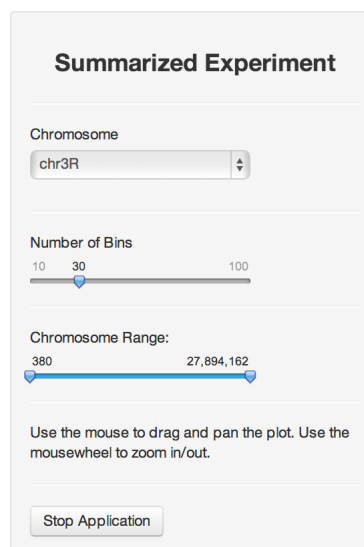
Figure 30: RangedSummarizedExperiment UI
