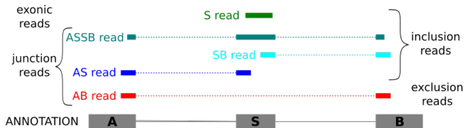
Figure 2: Different categories of reads. In this figure, we show an example of an alternative skipped exon. AS reads correspond to reads spanning the junction between the excluded sequence and its left flanking exon, SB to reads spanning the junction between the excluded sequence and its right flanking exon, ASSB to reads spanning the two inclusion junctions, S to reads entirely included in the alternative sequence and AB to reads spanning the junction between the two flanking exons. S reads correspond to exonic reads and all other categories of reads represented here correspond to junction reads.
