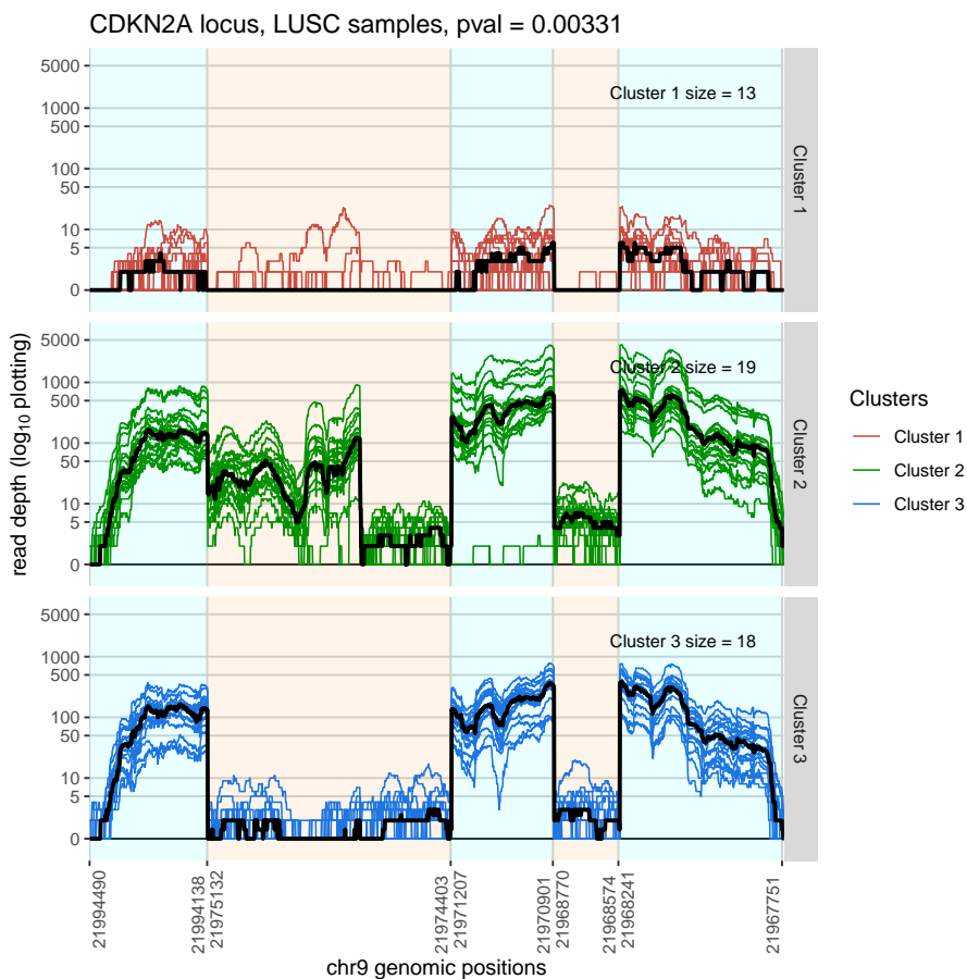
Figure 3: Graphical output from SFfigure for lplots=3 .
