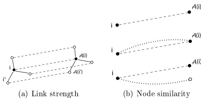
Figure 2: (a) The local link score S^l_{i, \mathcal{A}(i)} evaluates all pairwise similarities between links a_{ii'} and b_{\mathcal{A}(i)\mathcal{A}(i')} (solid lines) for a given pair of aligned nodes. (b) The local node similarity score S^n_{i, \mathcal{A}(i)} evaluates the overlap of the alignment with the node similarity R_{i, \mathcal{A}(i)} (dotted line). Top to bottom: Aligned node pairs (i) without similarity to any other node, (ii) with mutual node similarity, (iii) with (at least one) node similarity mismatch.
