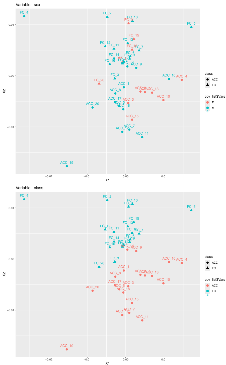
Figure 8: MultiDimensional Scaling plot. An unsupervised MDS plot is drawn. Samples are colored according to 'sex' variable (upper panel) and 'class' (lower panel).
