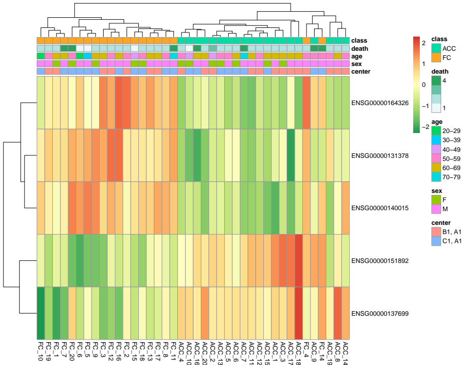
Figure 13: Clustergram. The clustergram is generated by using the expression values of the 5 predictors selected by DaMiR.FBest function. As for the heatmap generated by DaMiR.Allplot, 'class' and covariates are drawn as horizontal and color coded bars.
