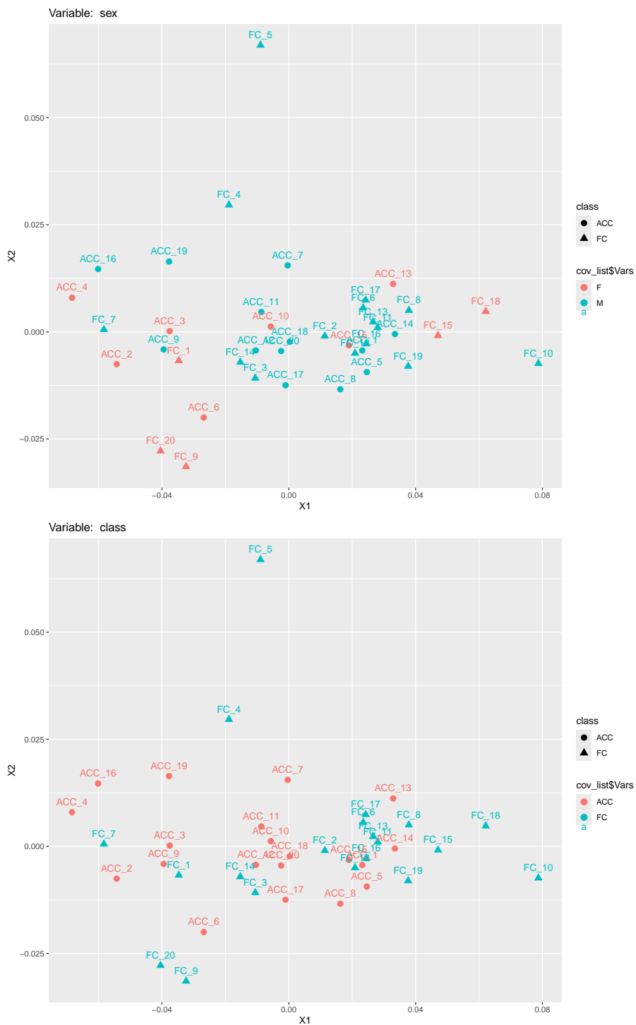
Figure 4: MultiDimensional Scaling plot. An unsupervised MDS plot is drawn. Samples are colored according to 'sex' variable (upper panel) and 'class' (lower panel).
